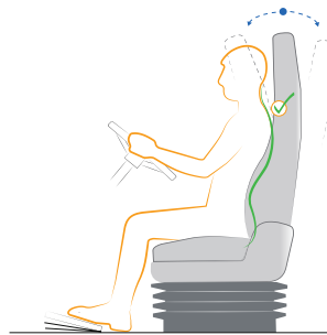
Pneumatisch entriegelbare Schulteranpassung Pneumatically releasable shoulder adjustment
